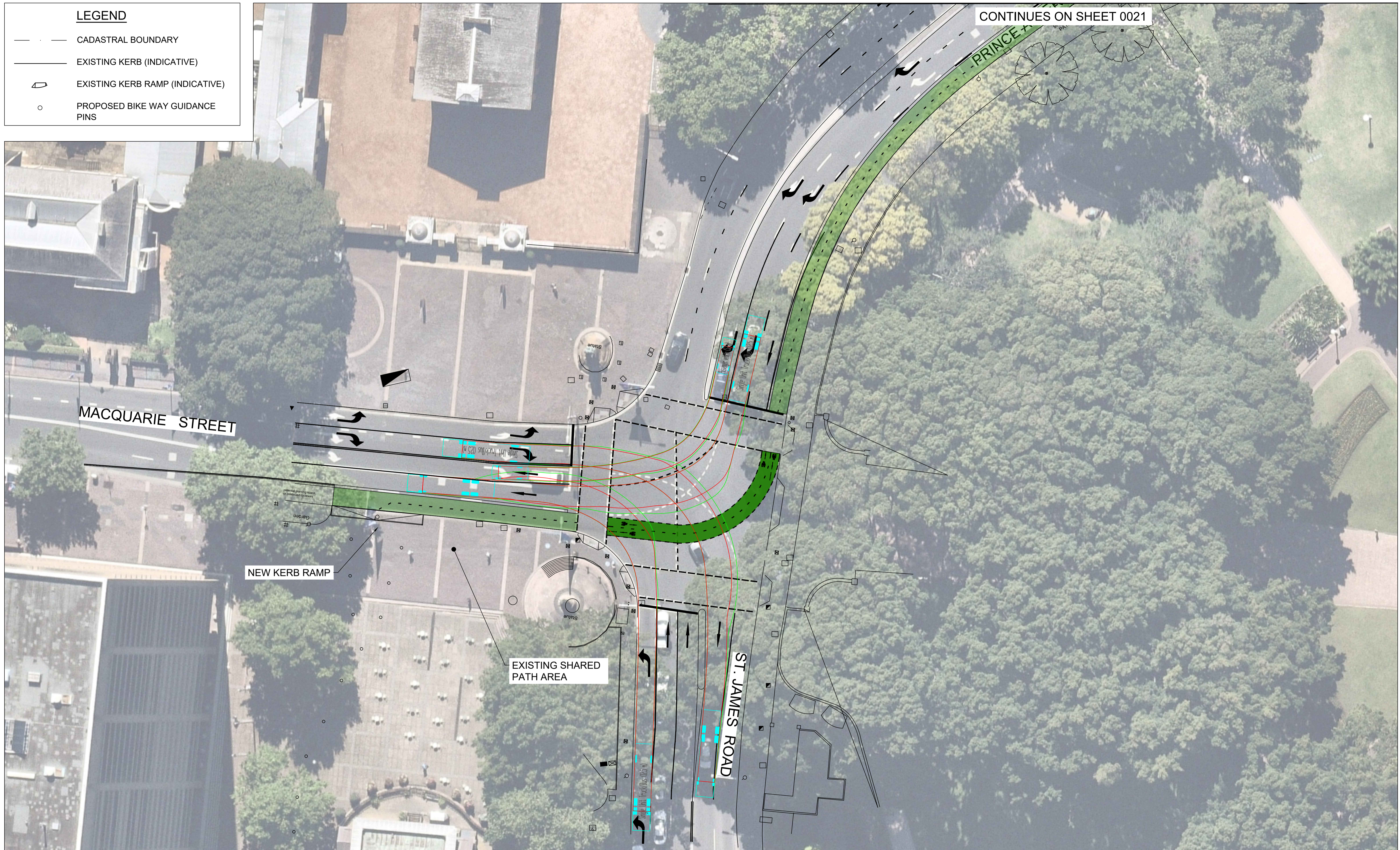
KING STREET EAST PLAN SCALE 1:250
